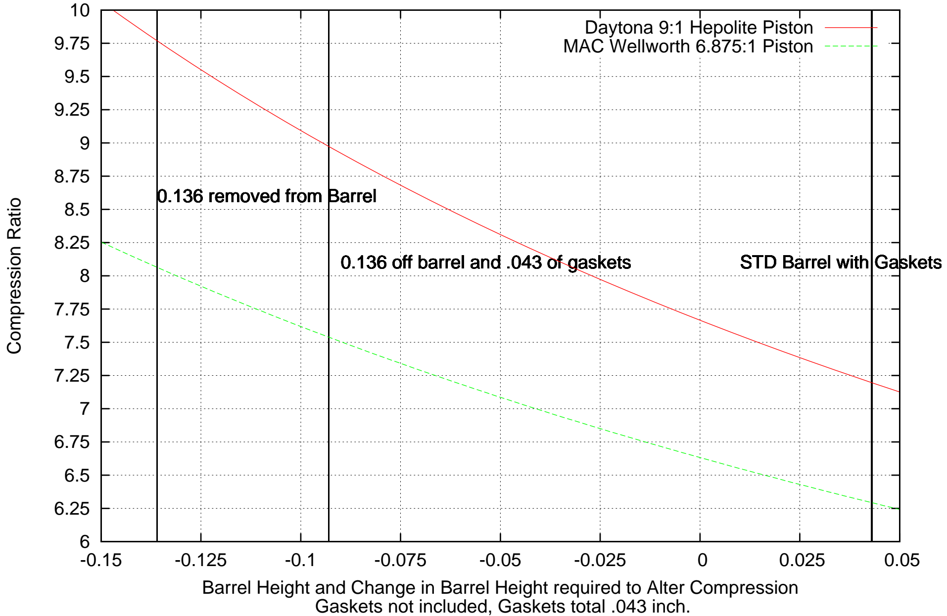
Compression Ratio vs Barrel Height and Gaskets/Compression Plates
